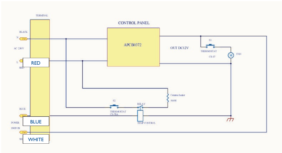
BIO-500F/120v Wiring Schematic
