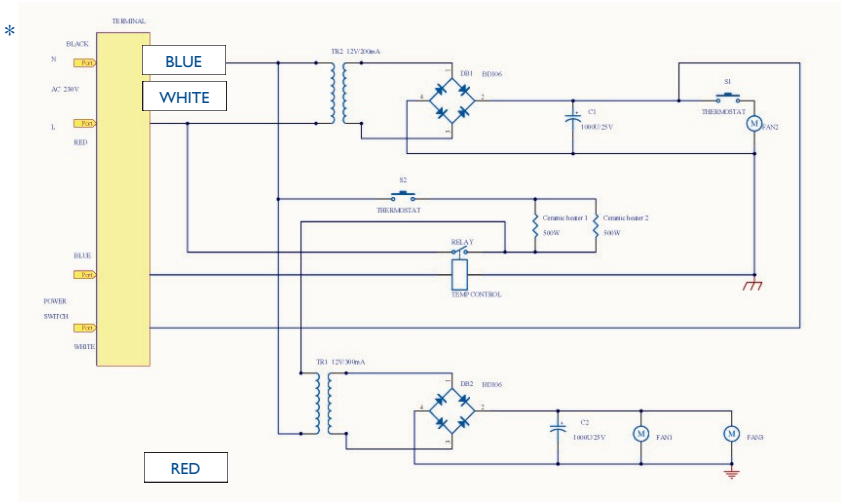
BIO-1000F/120v Wiring Schematic
